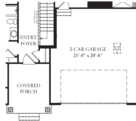
Craftsman Elev. @ Opt. 2' Garage Extension
